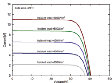
I-V Curves of 365M at different irradiance
