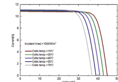
I-V Curves of 365M at different cell temperature
